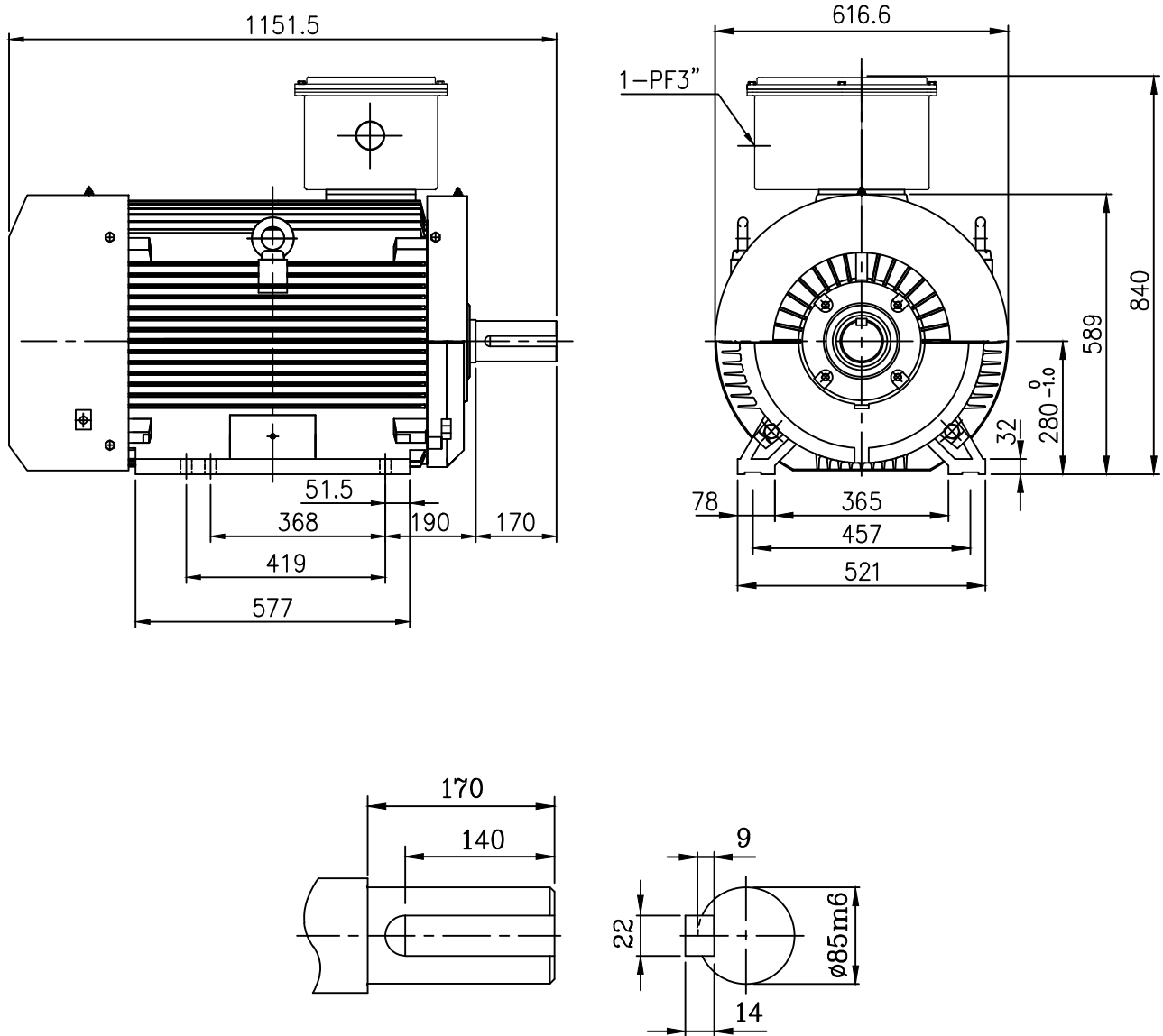
SHAFT EXTENSION
